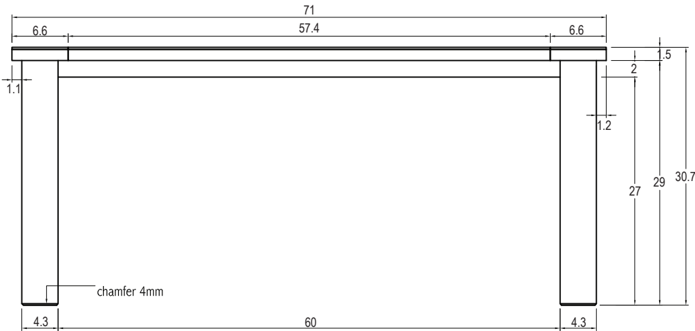
FRONT VIEW / VUE DE FACE / VISTA FRONTAL
